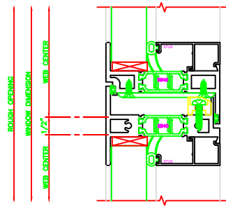
533 MEETING RAIL 325 CASEMENT IN / FIXED BUTT HINGES
